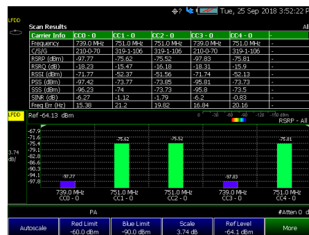
Multiple carrier frequencies measurements with strong cell display
