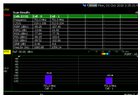
Multicell measurement with cell ID on single carrier frequency
