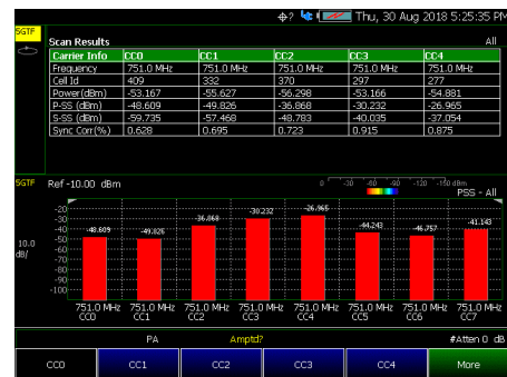
5GTF OTA supports Verizon's pre-5G networks and measures control channels and displays cell ID
