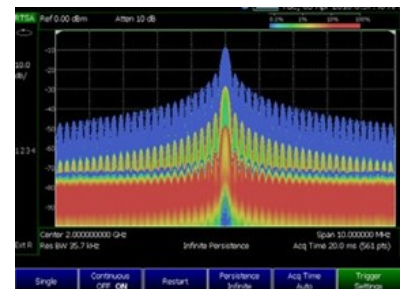
Multi-pulse detection using density display with settable persistence
